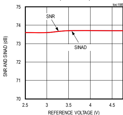
SNR AND SINAD vs. REFERENCE VOLTAGE (CHANNEL B)
