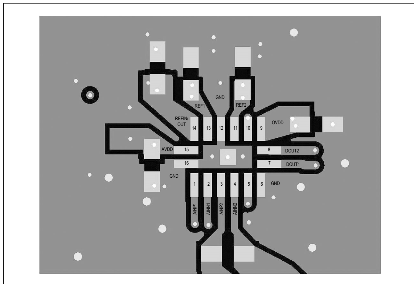
Figure 15. PCB Layout Example for MAX11192
