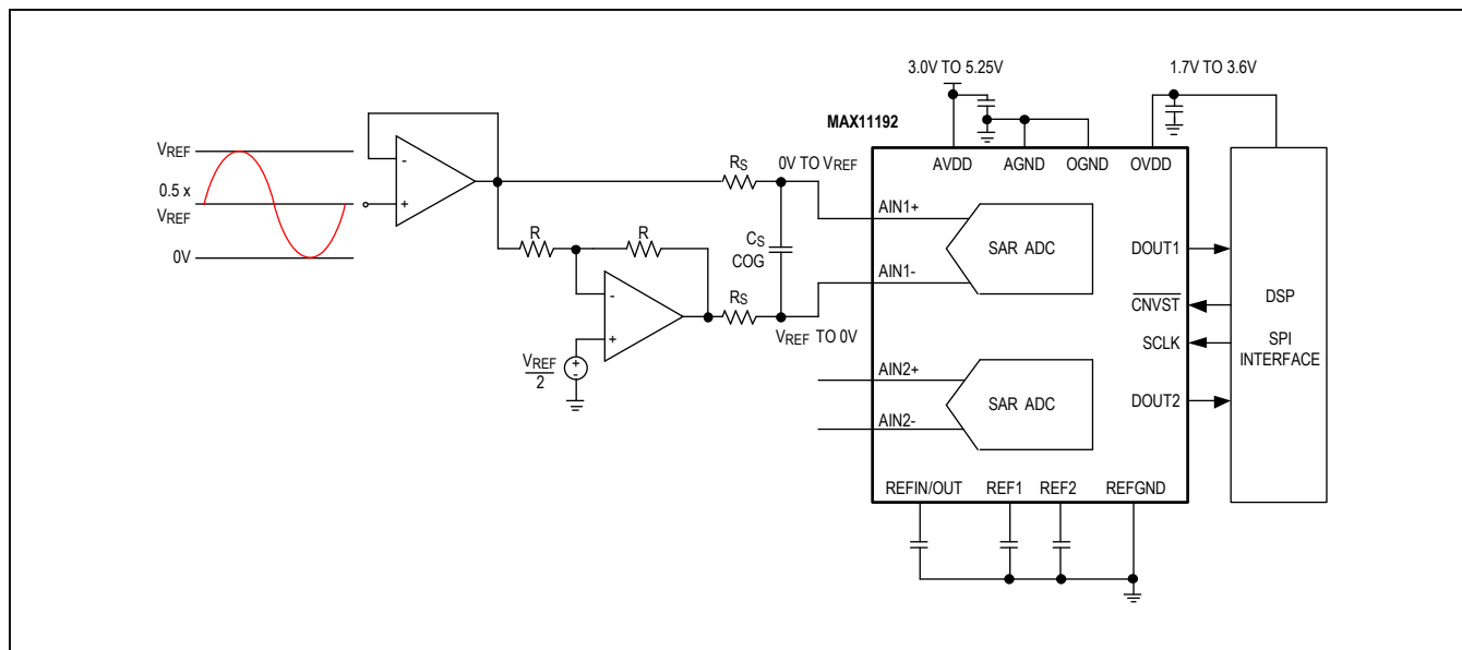
Figure 13. Unipolar Single-Ended Input
