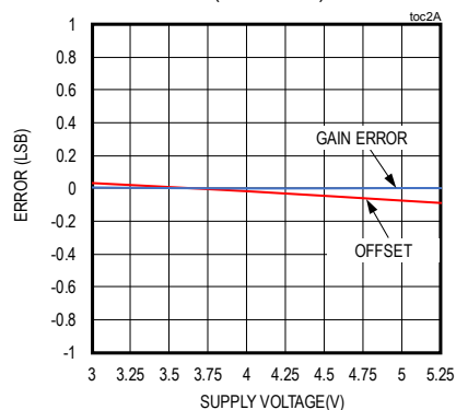
OFFSET AND GAIN ERROR vs. SUPPLY VOLTAGE (CHANNEL A)
