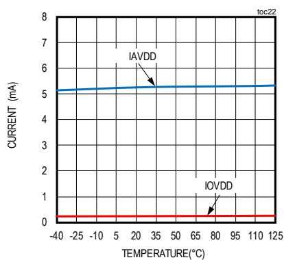
CURRENT vs. TEMPERATURE
