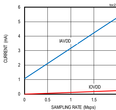
CURRENT vs. SAMPLING RATE
