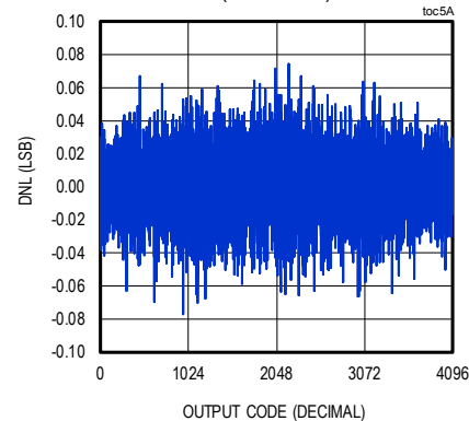
DNL vs. CODE (CHANNEL A)
