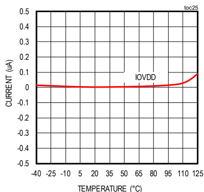
OVDD STANDBY CURRENT vs. TEMPERATURE
