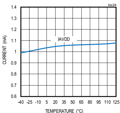
AVDD STANDBY CURRENT vs. TEMPERATURE
