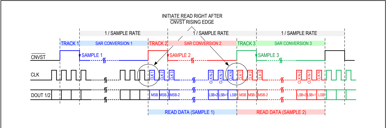
Figure 7. Convert and Data Read MAX11192
