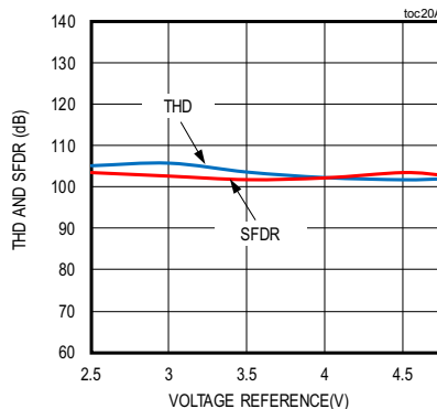
THD AND SFDR vs. REFERENCE VOLTAGE (CHANNEL A)
