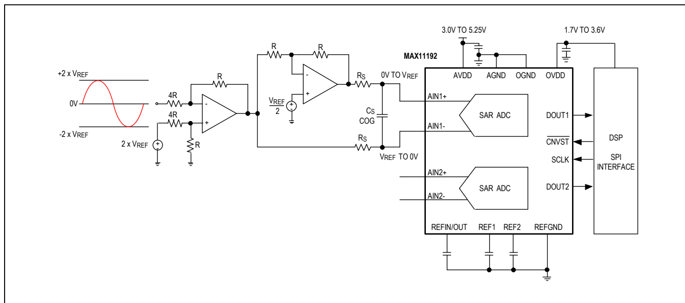
Figure 14. Bipolar Single-Ended Input
