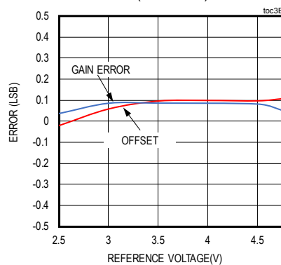
OFFSET AND GAIN ERROR vs. REFERENCE VOLTAGE (CHANNEL B)
