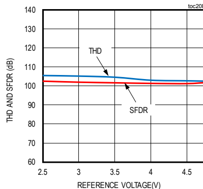
THD AND SFDR vs. REFERENCE VOLTAGE (CHANNEL B)
