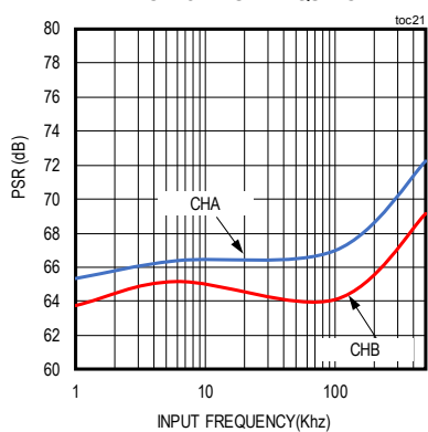
PSR vs. INPUT FREQUENCY
